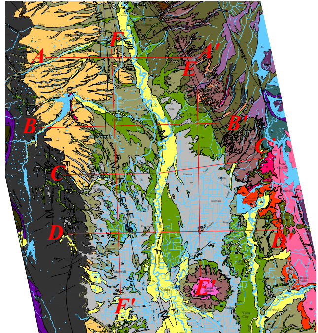
Figure 1. Northern Sacramento Valley Geologic Map. Red lines illustrate geologic cross-sections used in investigations of the northern Sacramento Valley aquifer systems since 1997. The legend of corresponding geologic map units and names is below.
